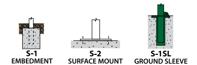
MOUNTING OPTIONS
